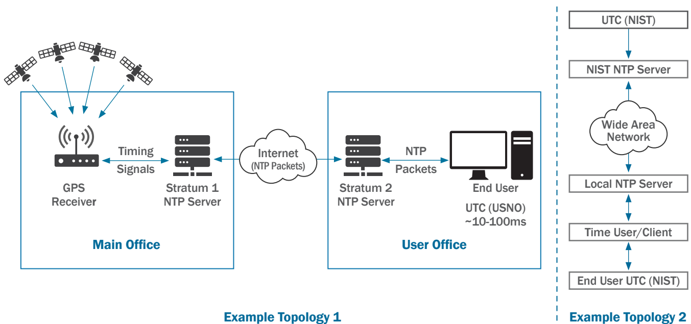
Figure 1: Topology Examples
